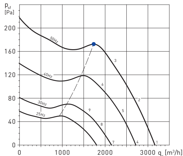
TD-4000/355 TRI
